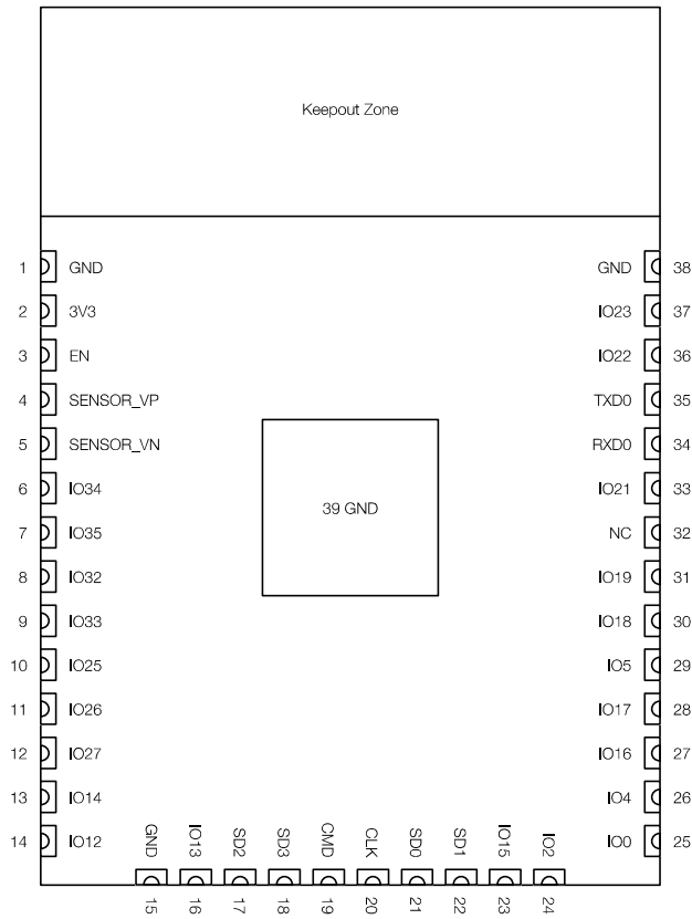
Figure 1: ESP32-WROOM-32D Pin Layout (Top View)
